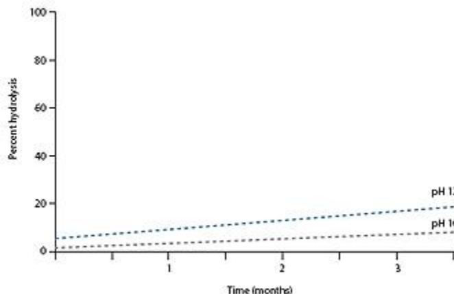
Hydrolytic stability of Gafquat HS-100 polymer at pH 10 and pH 12 at 45°C
